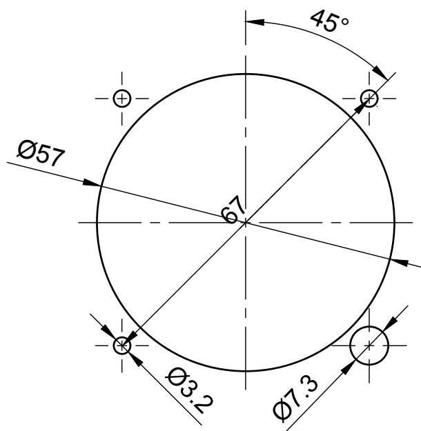
Cutout Drawing
